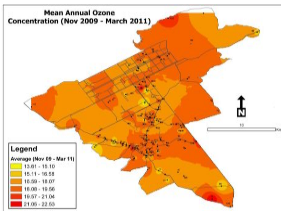
Fig.1. Spatial distribution of O_3 conc. in Rawalpindi/Islamabad.
