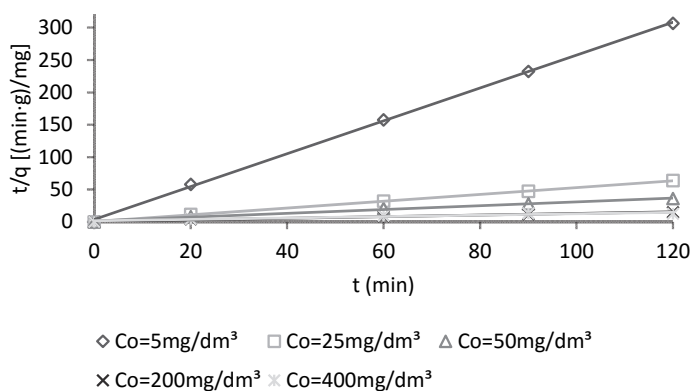
Fig. 7. Effect of initial Cu^{2+} concentration in solution on the reaction rate constant
