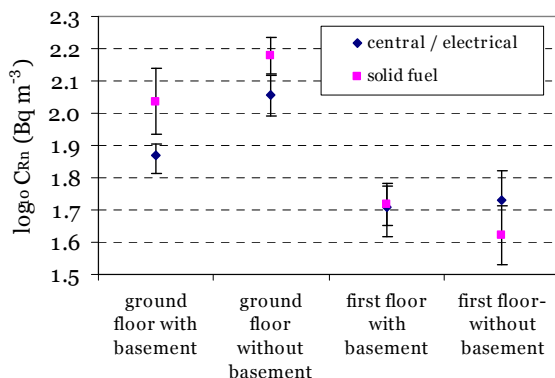
Figure 4. Influence of type of heating on indoor radon concentration, measured as function of floor level and presence or absence of basement
