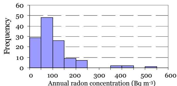
Figure 2 Histogram of the annual indoor radon concentration
