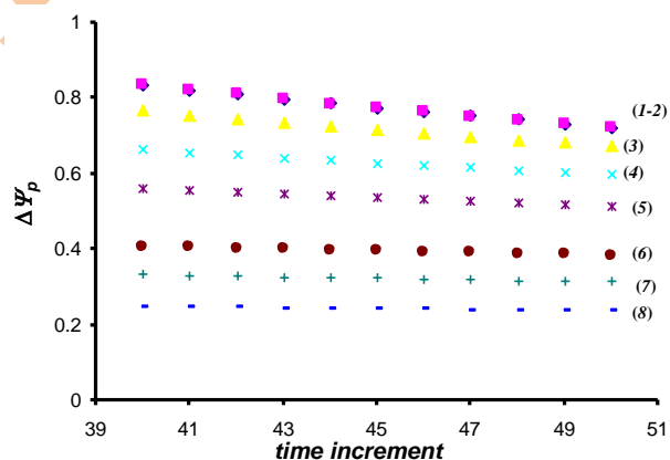
Fig. 3. Quasireversible electrode reaction of a dissolved redox couple. Variation of the net peak current of voltammograms constructed by sampling the currents at different time increments of potential pulses versus time increments, for the electrode kinetic parameter \log(\kappa) : 2.15 (1); 1.15 (2); 0.15 (3); -0.15 (4); -0.35 (5); -0.65 (6); -0.85 (7), and -1.8 (8). The other conditions of the simulations are identical as for Fig. 2.
