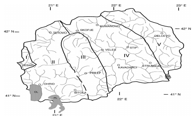
Figure 1. Major tectonic units of Macedonia. I. Chukali-Krasta unit; II. Western Macedonian unit; III. Pelagonian massif; IV. Vardar zone; and V. Serbian - Macedonian massif. Lakes: DL—Dorjan Lake, OL—Ohrid Lake, and PL—Prespa Lake
