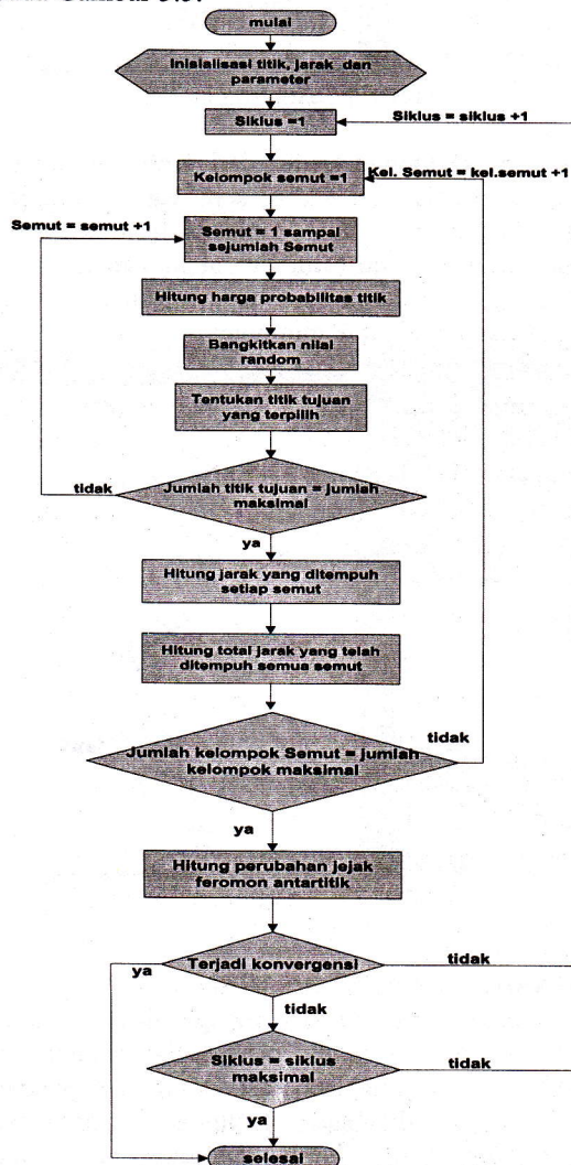
Gambar 3.5 Flowchart Algoritma Ant System
