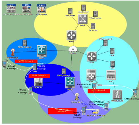
Fig. 4 - Integrated heterogeneous scenario
