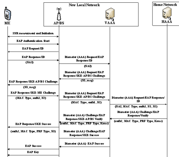
Fig.5 Message flow during vertical handover scenario
