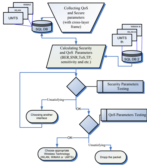
Fig. 2 – Illustration of SQoSXIP Module algorithm
