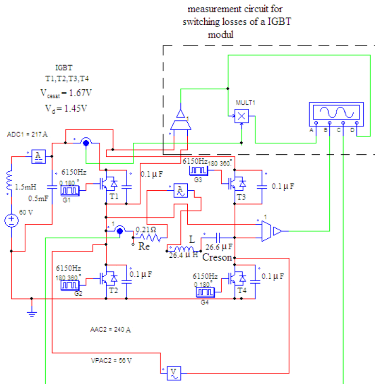
Fig. 2. Simulation circuit of the full bridge serial resonant power converter and circuit to measurement of the switching losses of a IGBT transistor in PowerSim simulation program
