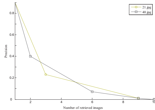
Fig. 2. Relationship between precision and the number of retrieved images for the images 21.jpg and 40.jpg
