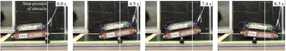
Figure 11. Climbing-over motion of Kenaf over unfixed obstacle with diameter D = 33 [mm] on slope \phi = 0 [°]
