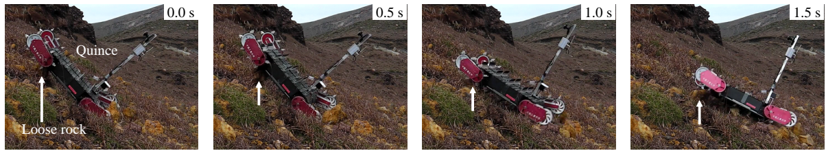
Figure 1. Tracked robot "Quince" sliding down owing to rolling of loose rocks at Mt. Aso
