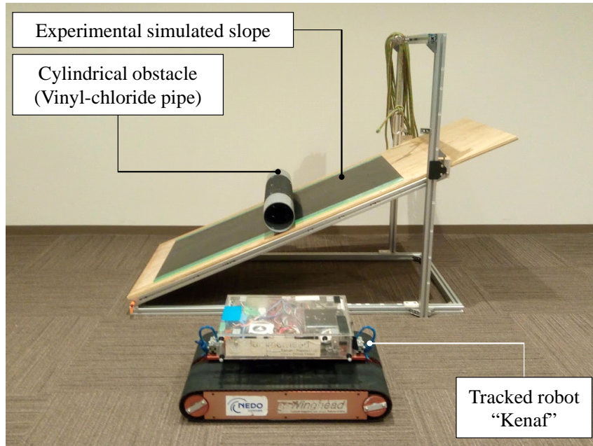
Figure 5. Experimental equipments
