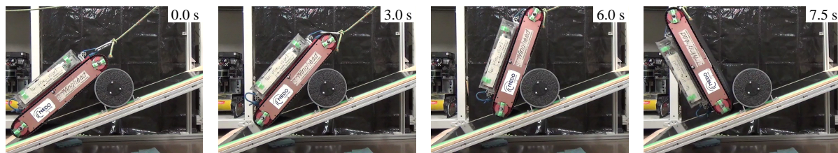
Figure 9. Tipping-over motion of Kenaf over fixed obstacle with diameter D = 166 [mm] on slope \phi = 20 [°]
