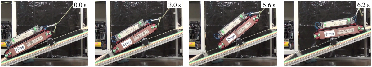
Figure 7. Climbing-over motion of Kenaf over fixed obstacle with diameter D = 61 [mm] on slope \phi = 20 [°]
