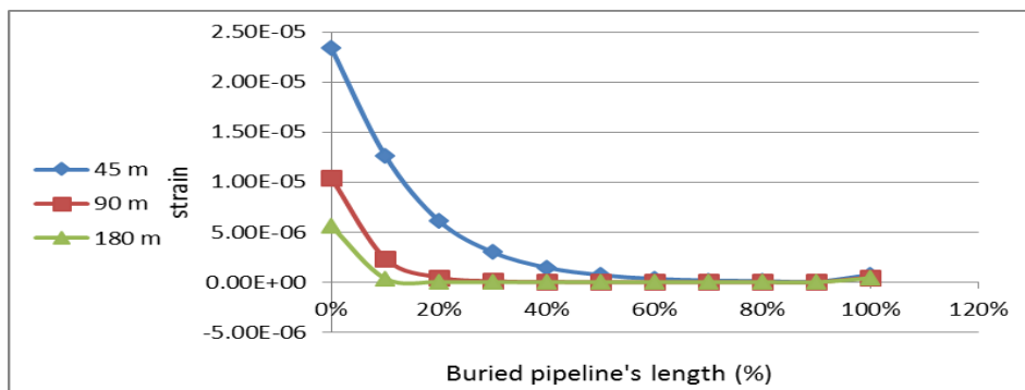
Fig. ( 8 ) Strains–percentage of buried pipeline's length relationship for different values of length.
