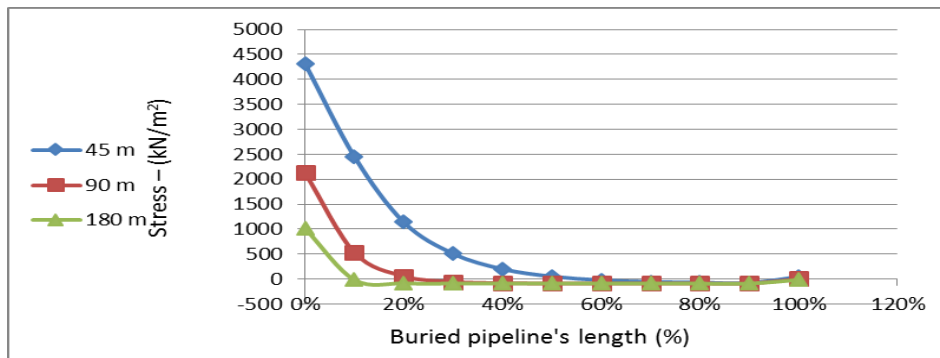
Fig. ( 7 ) Stresses–percentage of buried pipeline's length relationship for different values of length.
