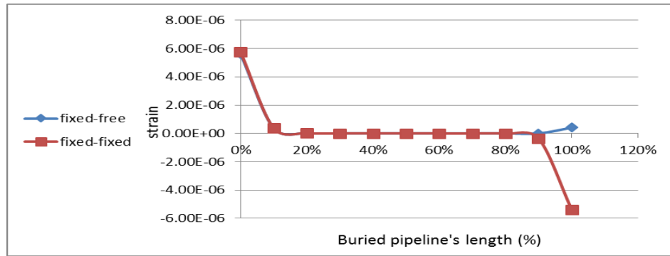
Fig. 17 Strain–percentage of buried pipeline's length relationship for two ends conditions.
