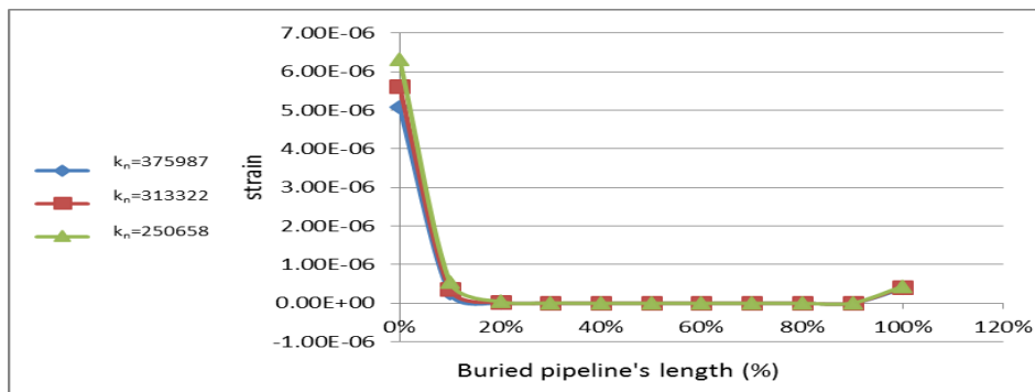
Fig. (11) Strain–percentage of buried pipeline's length relationship for different values of ( k_n and k_s ).
