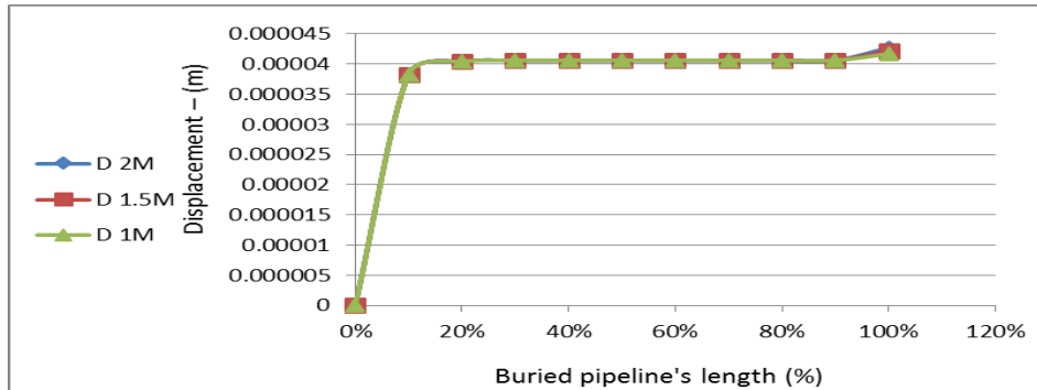
Fig. (12) Displacement–percentage of buried pipeline's length relationship for different values of depth of soil cover.
