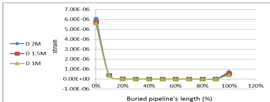
Fig. (14) Strain–percentage of buried pipeline's length relationship for different values of depth of soil cover.
