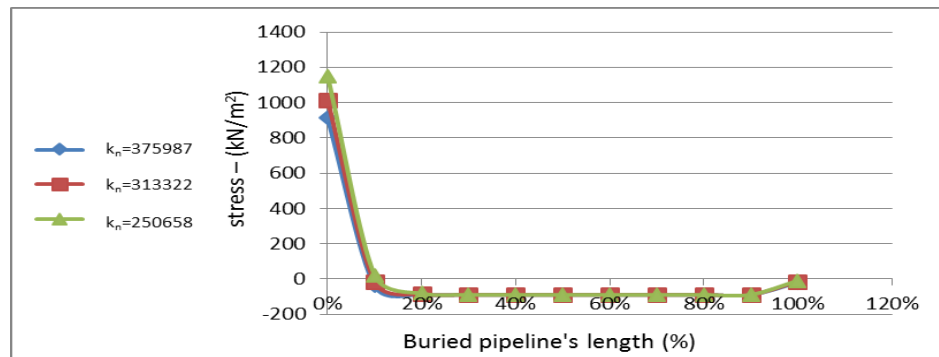
Fig. ( 10 ) Stresses–percentage of buried pipeline's length relationship for different values of ( k_n and k_s ).
