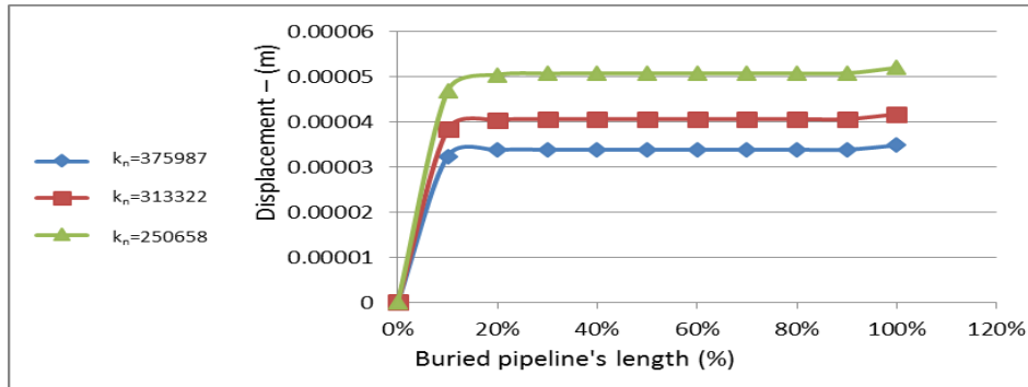
Fig. ( 9 ) Displacement–percentage of buried pipeline's length relationship for different values of ( k_n and k_s ).
