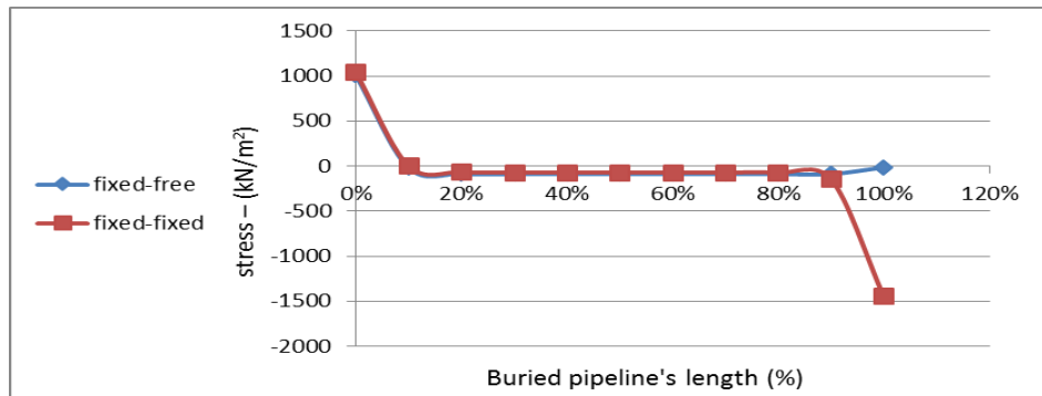
Fig. (16) Stresses–percentage of buried pipeline's length relationship for two ends conditions.
