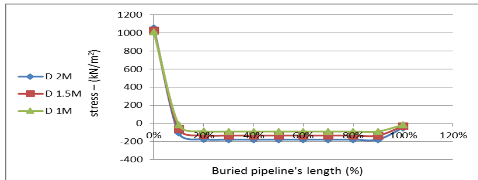
Fig. (13) Stresses–percentage of buried pipeline's length relationship for different values of depth of soil cover.
