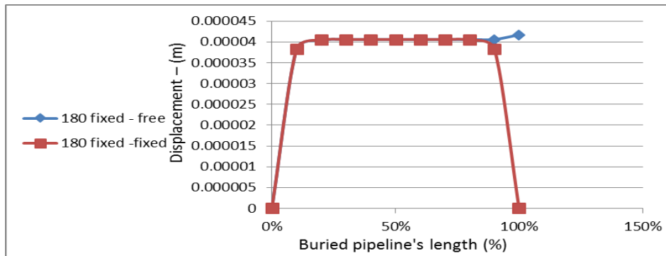
Fig. (15) Displacement–percentage of buried pipeline's length relationship for two ends conditions
