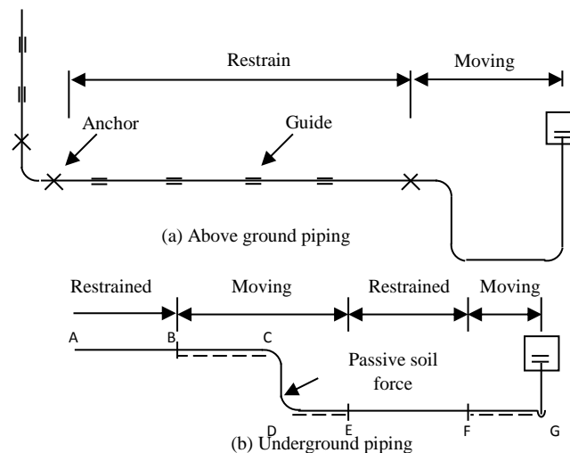
Fig. ( 1 ) Restrained and moving portions of a pipeline.
