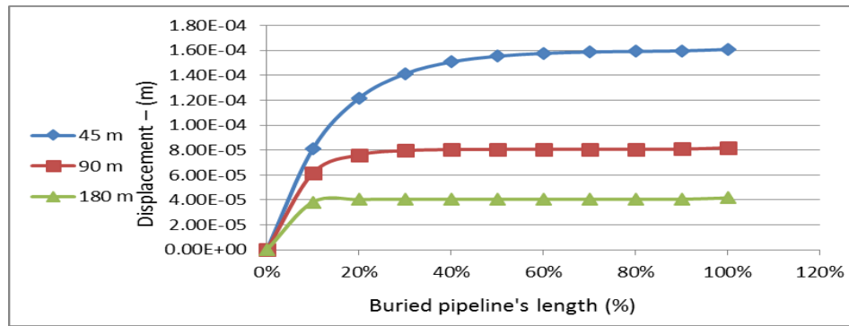
Fig. ( 6 ) Displacement–percentage of buried pipeline's length relationship for different values of length.
