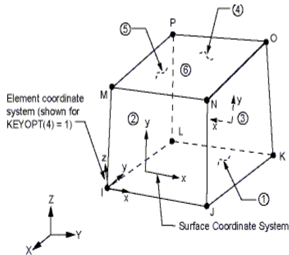
Fig. (2) Solid45, (3-D) buried pipeline element.
