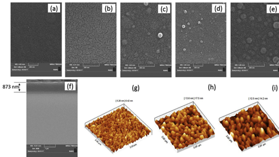
Figure 4. Morphological evaluation of Cu/a-C:H thin coating. SEM of the a (T-1) b (T-2) c (T-3) d (T-4) e (T-5) f (cross section of T-1. AFM image of (g) T-1, (h) T-3 and (i) T-5.
