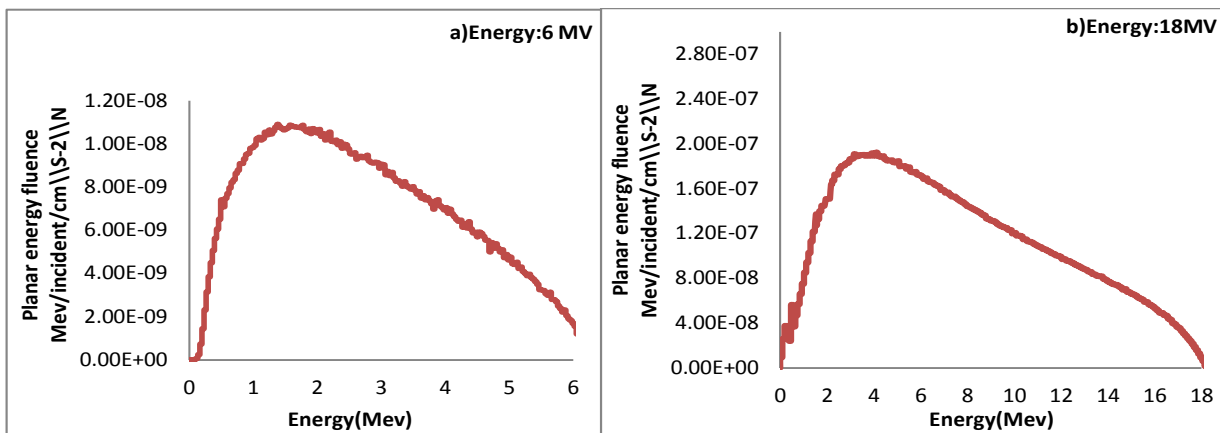
Figure 5: Photon energy fluence spectra for the reference 10x10 cm 2 field size at 10 cm depth on the central axis, for the 6 (a) and 18 (b) MV photon beams. The plotted spectra are normalized to the total incident photon energy fluence \phi_0 by using Equation (4).
