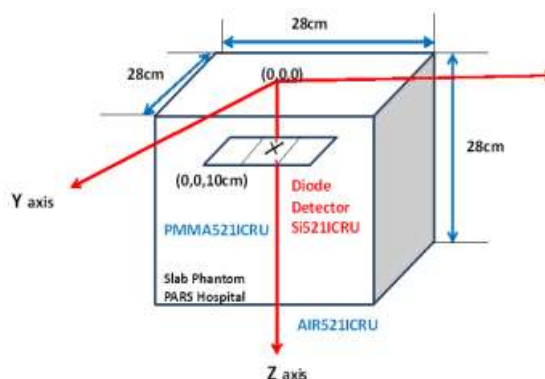
Figure 2: The phantom used to model the diode detector in the PMMA medium using DOSXYZnrc MC code.
