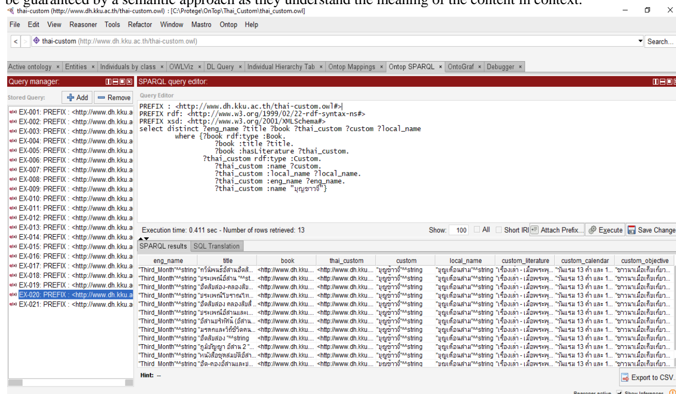
Figure 8. Running SPARQL queries through on top SPARQL
