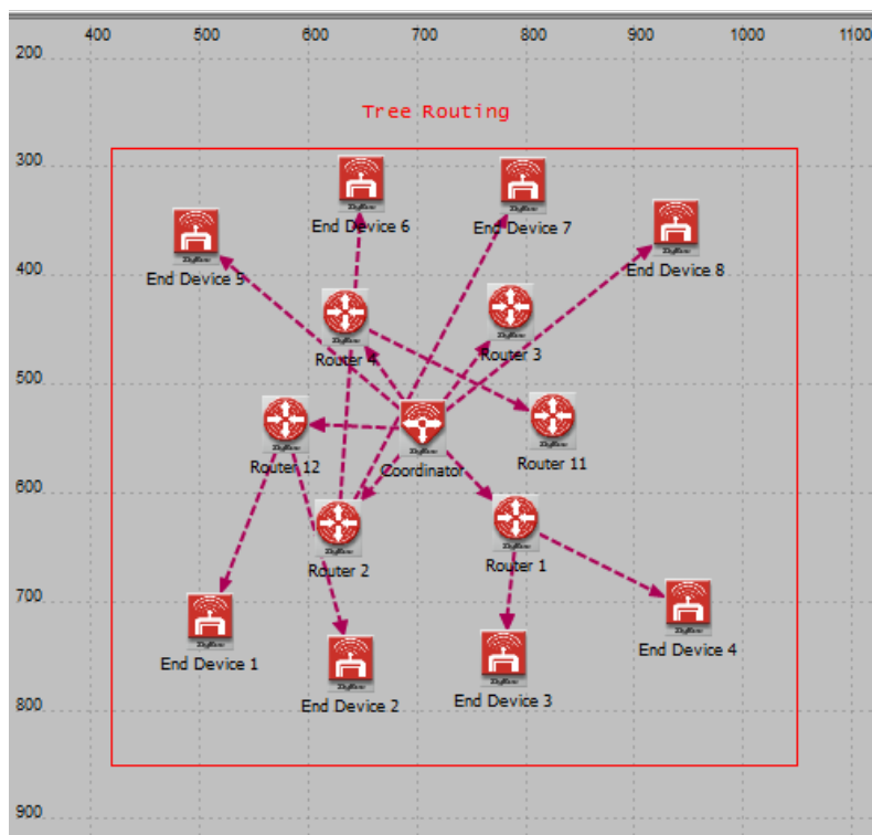
Figure 3. Tree routing
