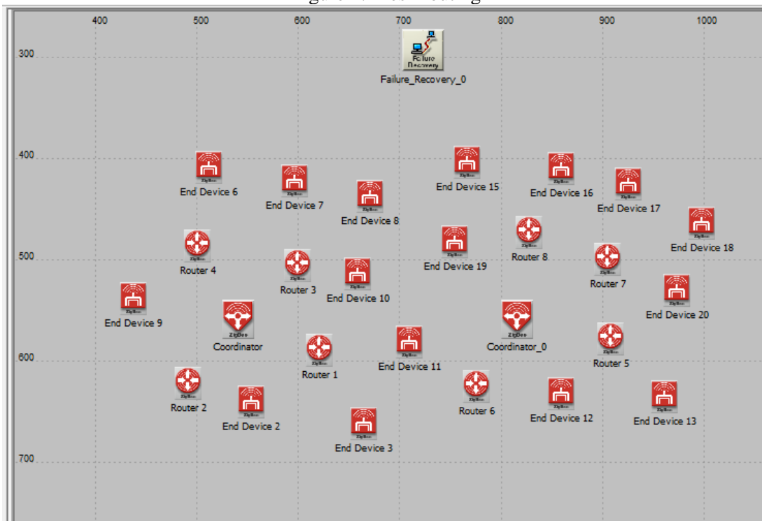
Figure 5. Coordinator failure
