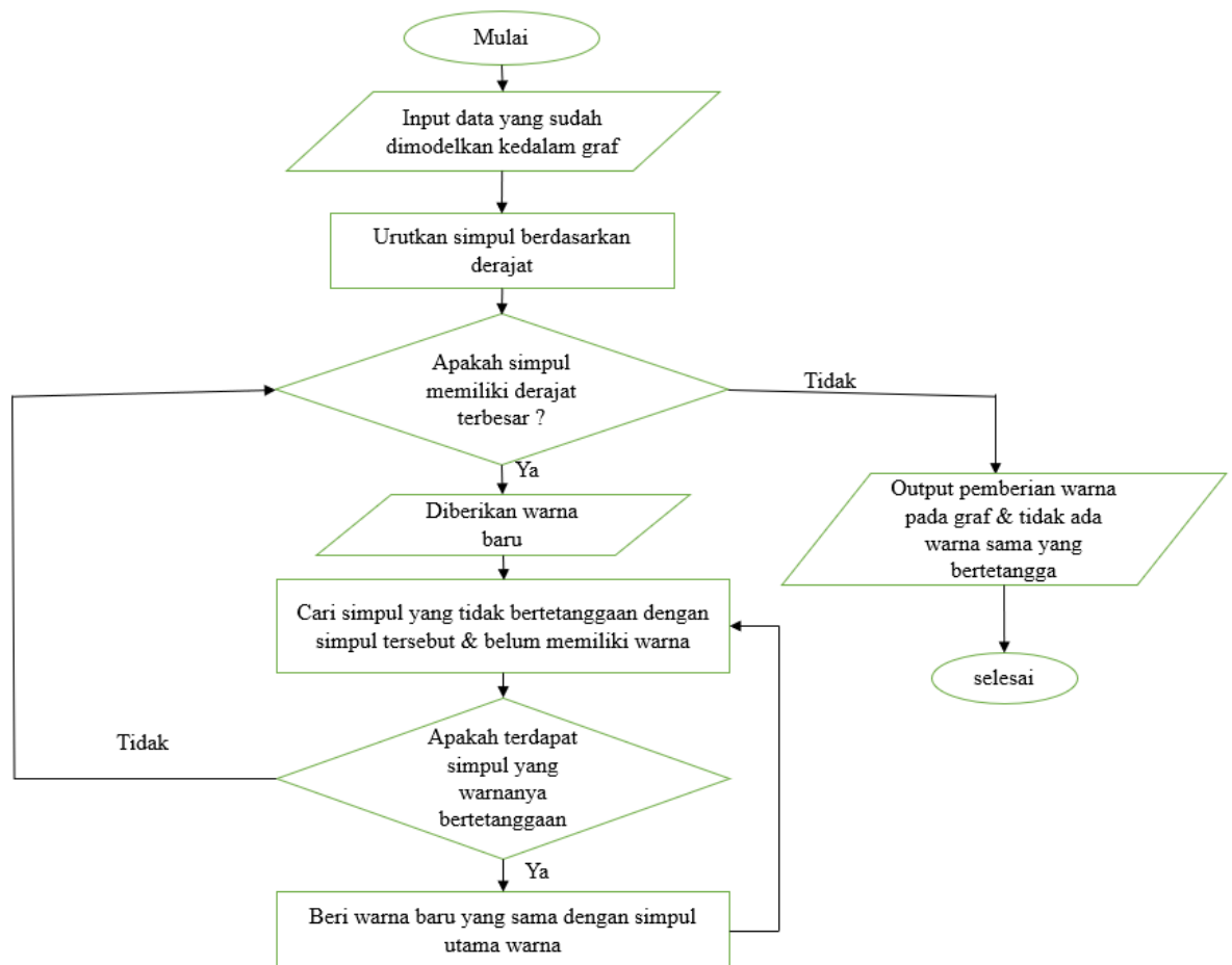
Gambar 3.2. Flowchart Algoritma Welch-Powell
