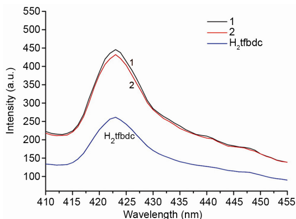
Fig. 7—Solid-state emission spectra for free ligand \text{H}_2\text{tfdc} and complexes 1 and 2 ( \lambda_{\text{ex}} = 370 nm) at room temperature.
