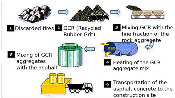
Figure 4. Wet process (Villamizar, 2016).
