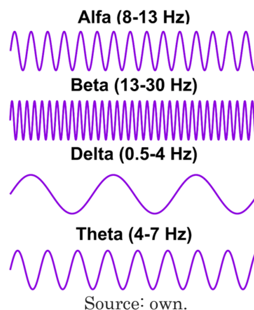
Figure 1. Representation of bands of the electroencephalogram.
