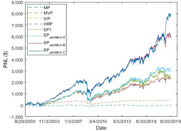
Figure 6.5 PNL curves of MVP, MP, IVP, HRP, EP1 and EP_{\text{partition A}} , EP_{\text{partition B}} , EP_{\text{partition C}} for EOD returns of the most allocated 10 stocks in sector ETFs XLE, XLF and XLU from Aug. 29, 2000 to Aug. 30, 2019 with W = 252 and \rho_{TH} = 0.45 . All portfolios are self-funded (available capital is always positioned) with initial investment of $1,000, rebalanced daily without any trading cost involved.
