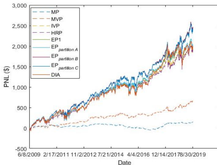
Figure 6.6 PNL curves of MVP, MP, IVP, HRP, EP1 and EP_{partition A} , EP_{partition B} , EP_{partition C} and DIA for EOD returns of 30 stocks in the index DJIA from June 8, 2009 to Aug. 30, 2019 with the parameters W = 252 and \rho_{TH} = 0.4 . All portfolios are self-funded (available capital is always positioned), with initial investment of $1,000, rebalanced daily without any trading cost involved.
