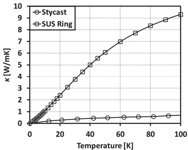
Figure 13. Measured, temperature-dependent thermal conductivity data for Stycast™ (2850GT) and SUS for the numerical models.
