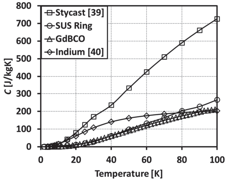
Figure 14. Measured, temperature-dependent specific heat data for Stycast™ (epoxy data from [39]), SUS, GdBCO with 15 wt% Ag and indium [40] for the numerical models.
