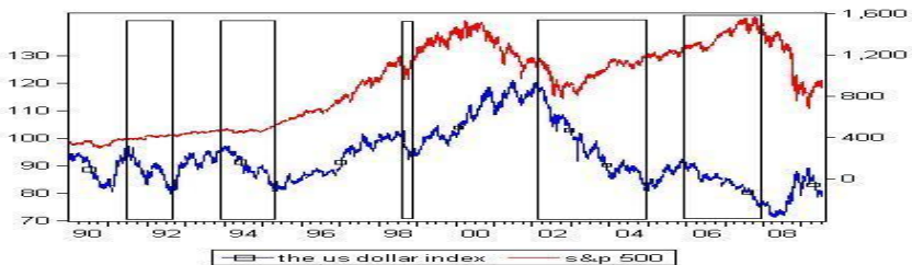
Figure 3: The chart of US dollar index and S&P 500 index from 1990.
