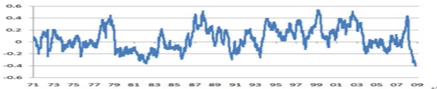
Figure 1: 6-Mth rolling Correlation of the Daily % Change of S&P 500 and US Dollar
