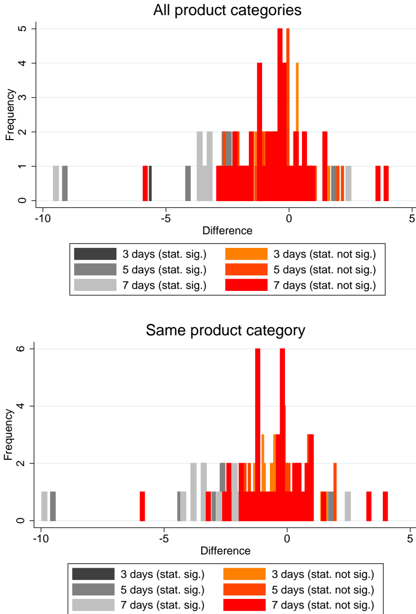
Figure 3: Differences in shopping bag additions between existing products recommended by new products and all other products
