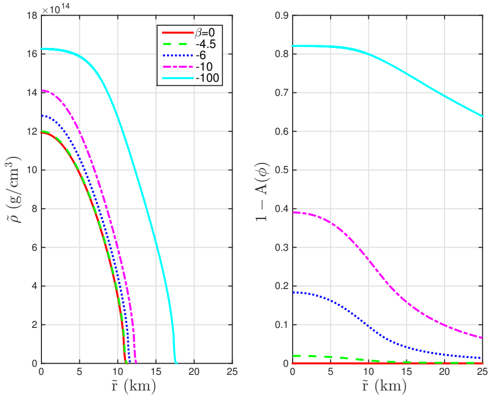
FIG. 1: Effect of varying \beta on the radial profiles of the matter density (left) and conformal factor 1 - A(\phi) (right) for neutron stars. The physical radius \tilde{r} = A(\phi(r))r is the radial coordinate associated with the Jordan frame metric. All cases have a fixed ADM mass of 1.70M_{\odot} , m_{\phi} = 1.6 \times 10^{-13}\text{eV} and HB EOS. The baryon mass of the neutron star is 2.06, 2.07, 2.10, 2.32, 5.37M_{\odot} for \beta = 0, -4.5, -6, -10, -100 respectively. Even for moderate values of \beta , the structure of the star is altered significantly. For large values such as \beta = -100 , observations of isolated stars might already be able to test spontaneous scalarization.
