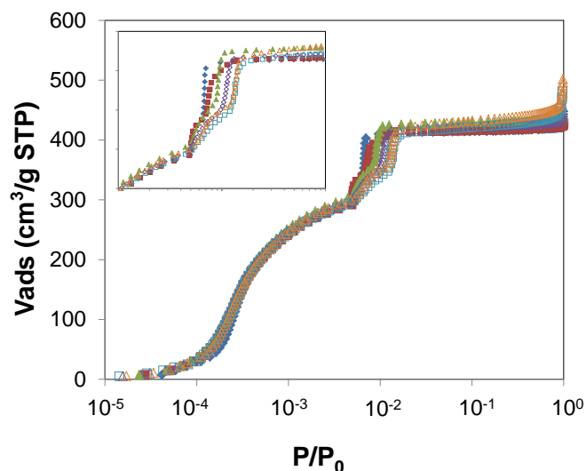
Fig. 3. Semi-log plot of N_2 adsorption isotherms at 77 K in ZIF-8 samples with different particle size. Blue closed diamonds, ZIF-8-98; red closed squares, ZIF-8-10; green closed triangles, ZIF-8-1.6; purple open diamonds, ZIF-8-0.61; blue open squares, ZIF-8-0.21; orange open triangles, ZIF-8-0.14.
