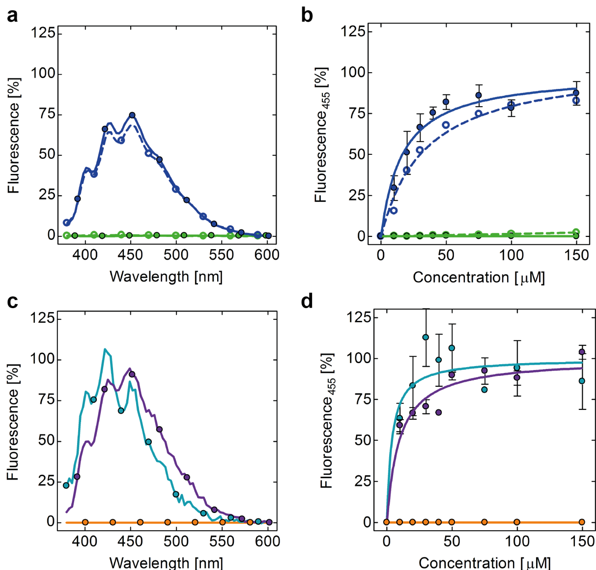
Figure 5. Accessibility of the channel of CC-Pent-T, CC-Hex-T and CC-Hept-T to the hydrophobic dye 1,6-diphenylhexatriene (DPH). (a and c) Fluorescence spectra of 1 \mu M DPH ( \lambda_{ex} = 350 nm) in the presence of 50 \mu M peptide. a) CC-Hex-T (blue, solid discs and continuous line), CC-Hex (blue, open circles and dashed line); CC-Tet2-F (green, solid discs and continuous line), and CC-Tet2 (green, open discs and dashed line). c) CC-Tri-F (orange, solid discs and continuous line), CC-Pent-T (turquoise, solid discs and continuous line), CC-Hept-T (purple, solid discs and continuous line). (b and d) Saturation binding at 455 nm of 1 \mu M DPH to varying concentrations of peptide. b) CC-9
