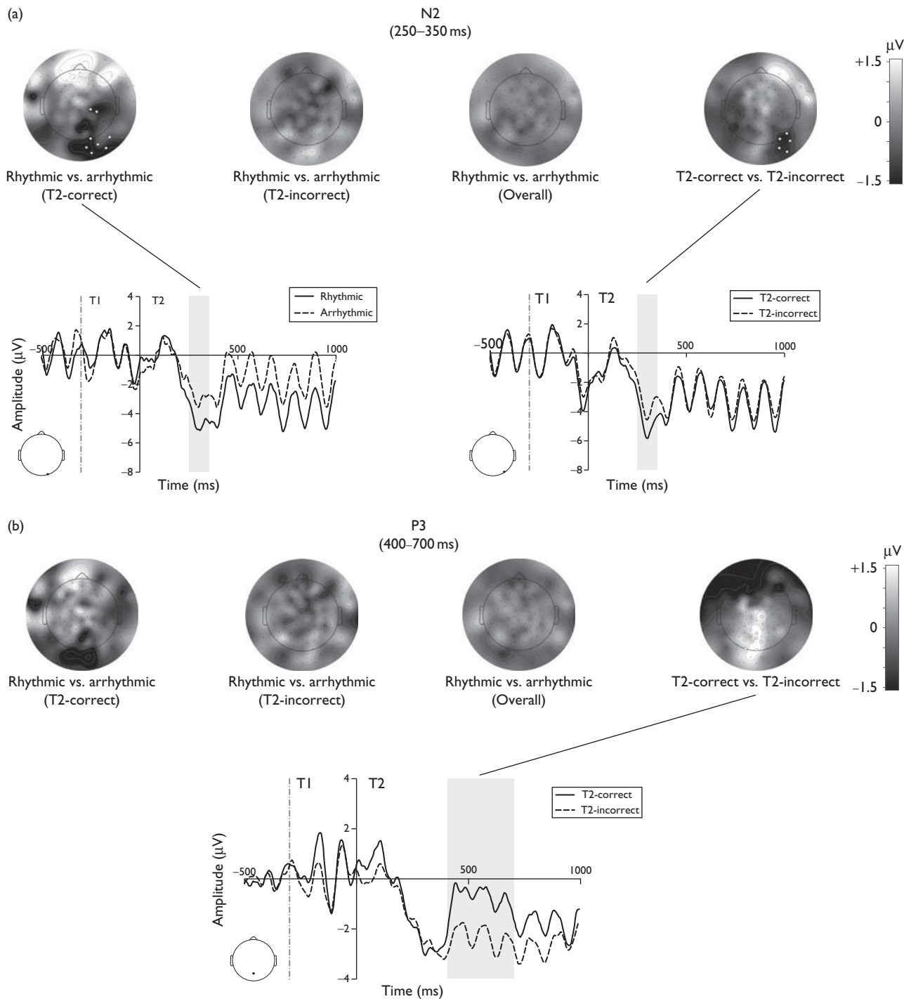
ERP results from experiment 1: N2 and P3 ERP components time-locked to the onset of T2. Scalp topographies for the difference in N2 (a) and P3 (b) between rhythmic and arrhythmic pre-RSVP conditions (divided for T2-correct, T2-incorrect and overall) and for the difference between T2-correct and T2-incorrect trials. Comparisons that were statistically significant (cluster-corrected permutation tests) are plotted with white-marked channels in their topographies and with ERPs waveforms of one representative channel underneath. Data are related to lag 3 trials. The same analyses for lag 8 can be found in Supplementary Fig. 1, Supplemental digital content 1, http://links.lww.com/WNR/A378 . ERPs, event-related potentials; RSVP, rapid serial visual presentation.
