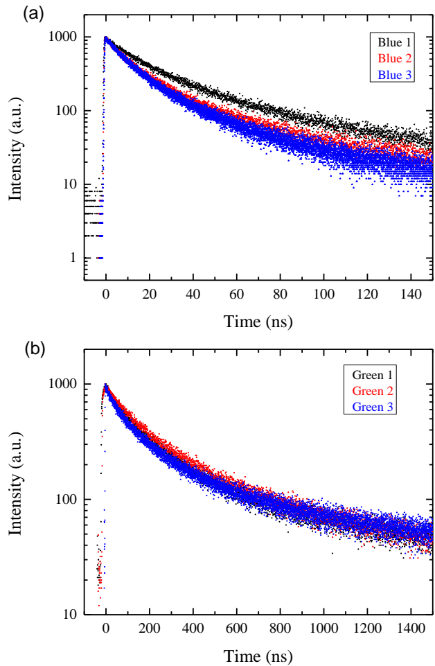
Figure 3 10 K PL decay transients detected at the PL emission peak for the (a) blue and (b) green emitting samples.
