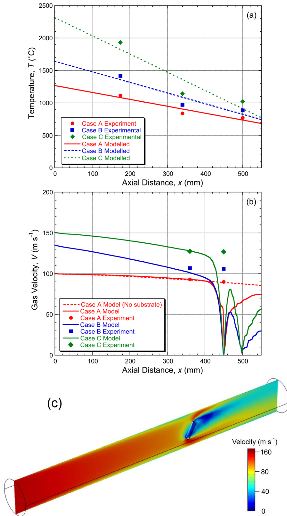
Fig.6 Experimental and modelled thermal and velocity fields of the gas, showing axial profiles for the three cases, with \theta = 90^{\circ} , of (a) temperature and (b) velocity, while (c) is a velocity contour map in the (vertical) x - r plane, for Case C, with \theta = 60^{\circ} , illustrating the perturbations caused by the substrate.
