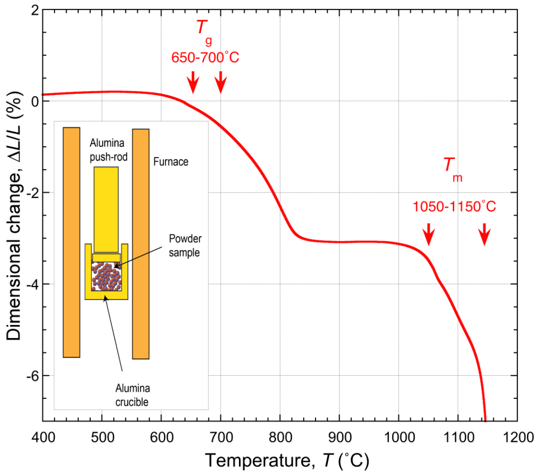
Fig.2 Fractional length change, as a function of temperature, for a compacted powder sample, obtained using a heating rate of 5\text{ }^{\circ}\text{C min}^{-1} .
