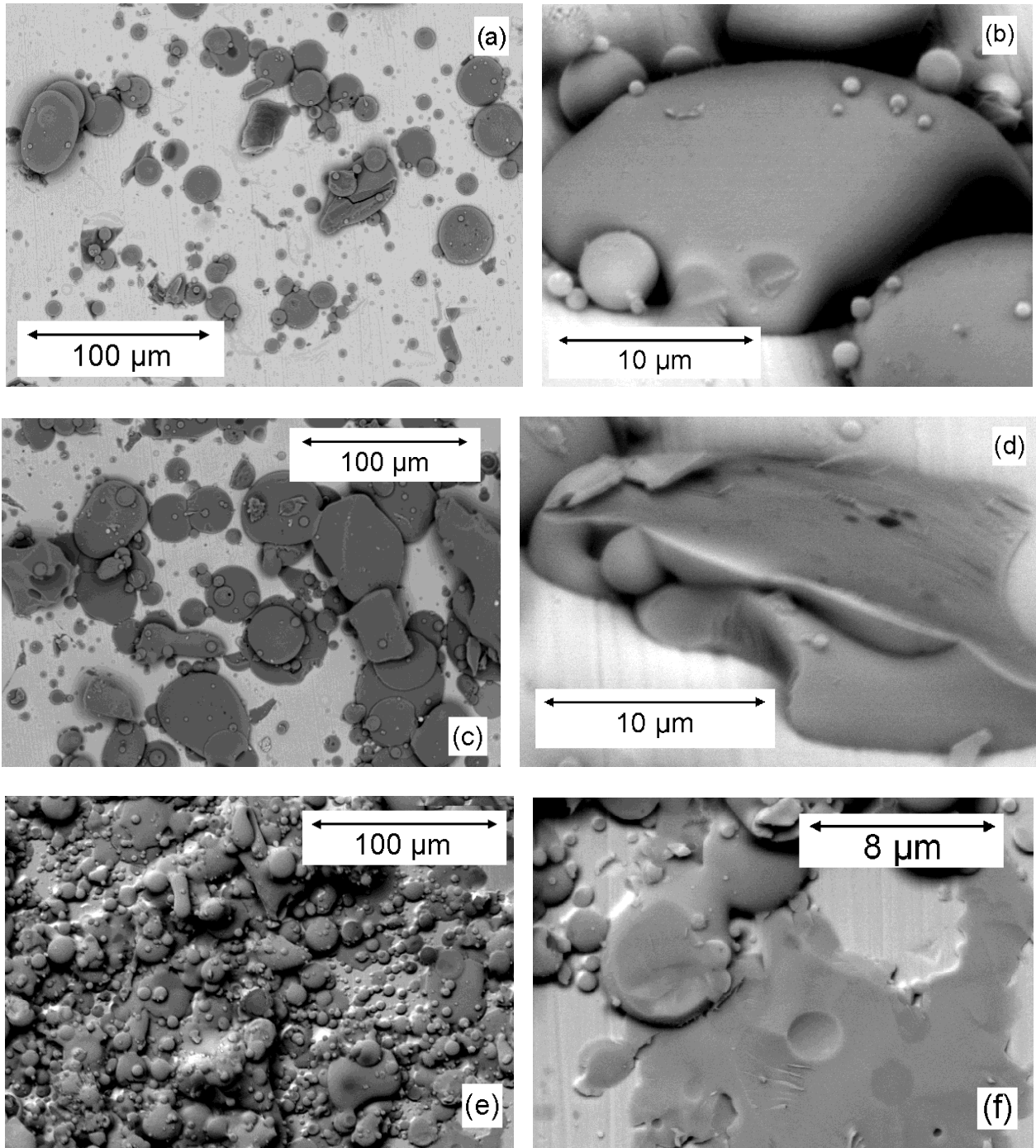
Fig. 8 SEM micrographs of insert surfaces, with adhering VA sputters, after powder injection for 10 s, with normal incidence ( \theta = 90^\circ ), under (a) & (b) Case A conditions, (c) & (d) Case B conditions and (e) & (f) Case C conditions.
