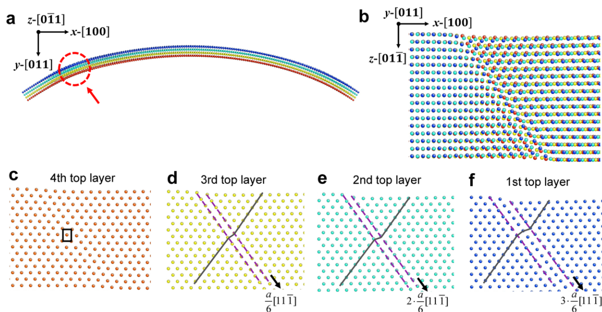
Figure 3. Illustration of a distorted \{110\} interface. (a) The snapshot of deformed nanowires at \theta = 26^\circ . The top four layers are present for each layer in a different color. The area indicated by the arrow is where the \{110\} interface forms. (b) Top view of atomic configuration in the area indicated by the arrow. (c)-(f) Atomic images for each top single layer from inside to the top of the nanowire.
