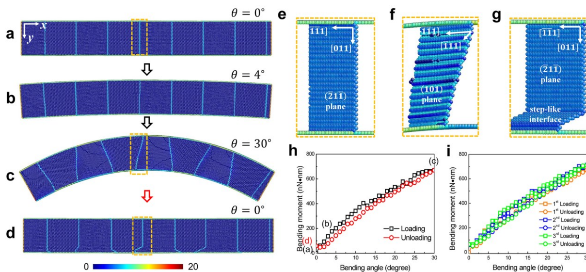
Figure 6. The bending of a \langle 111 \rangle / \{ 112 \} multi-twinned nanowire. (a)-(d) Typical atomic images for loading and unloading. (e)-(g) The interface morphology of different types in details. (h) The variation of bending moment with bending angle in the first bending cycle. (i) The variation of bending moment with bending angle in the first three bending cycles. The pseudo-elastic effect was fully recoverable under multiple cycling (after the first cycle when some defects were generated near the lower surface). The color of the atoms show their centrosymmetry parameter. [68]
