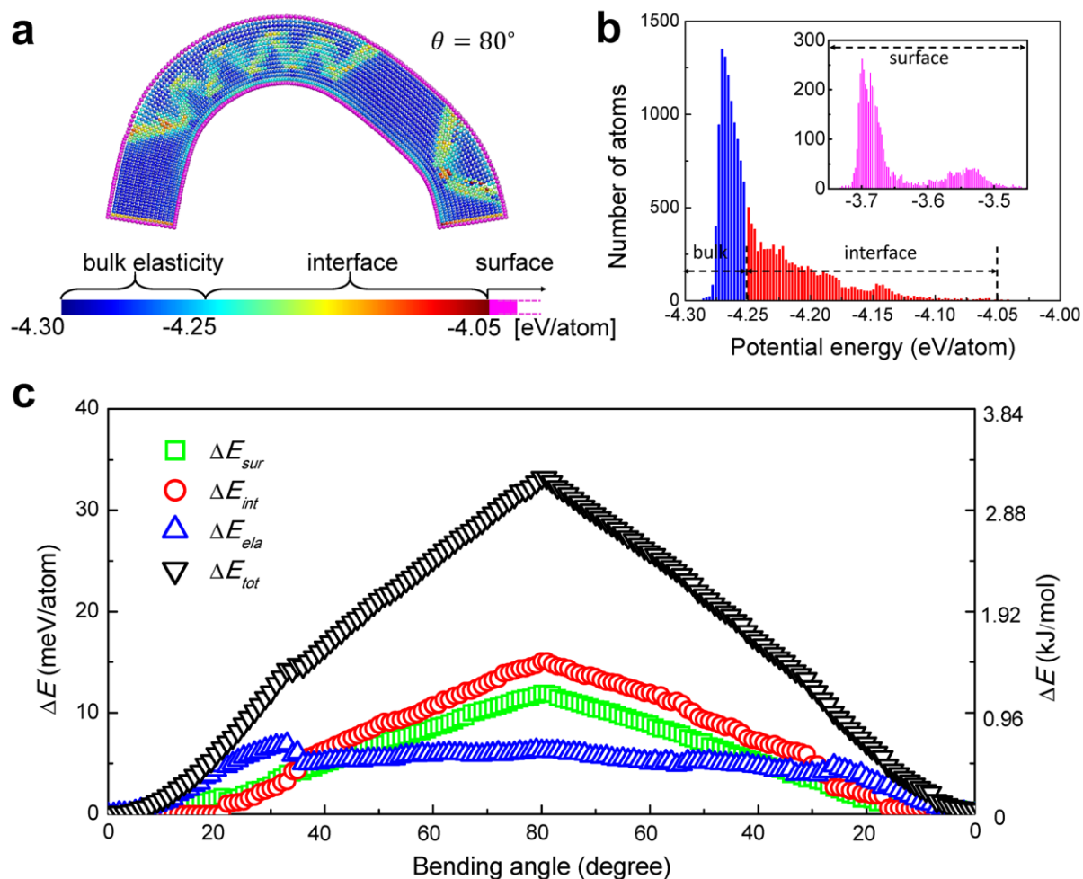
Figure 8. (a) Distribution of potential energy in a bent nanowire at \theta = 80^\circ (shown in Figure 2f). The colors show the atomic potential energy for each atom. (b) Distribution of atoms according to their potential energy. Three distinct energies are the elastic energy (blue), the interface energy (red) and the surface energy (magenta). Thresholds between the three groups were defined as -4.25 eV/atom (elastic to interfacial energy) and -4.05 eV/atom (interfacial to surface energy) (c) Variation of energy components upon loading and unloading. Red circle, blue triangle and green square represent \Delta E_{int} , \Delta E_{ela} and \Delta E_{sur} , separately. Black triangles represent the total potential energy as \Delta E_{tot} . The \{110\} interfacial energy provides the main driving force for shape recovery.
