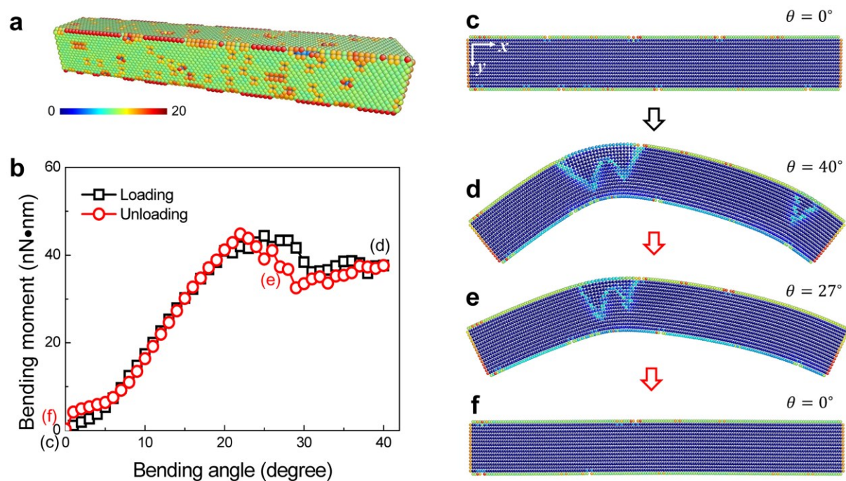
Figure 5. The effect of surface roughness on pseudo-elasticity. (a) The initial configuration of nanowires with rough surfaces. The color of the atoms is shown according to its centrosymmetry parameter. [68] (b) The variation of bending moment with bending angle. (c)-(f) Atomic configurations marked in (b).
