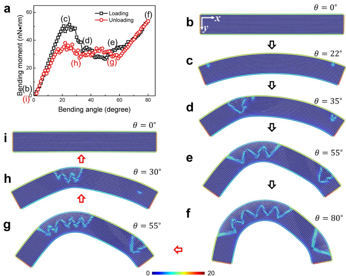
Figure 2. Pseudo-elasticity of \alpha -Fe nanowire ( 22.6 \text{ nm} \times 3.2 \text{ nm} \times 3.2 \text{ nm} ) under bending at 300 K. (a) The variation of bending moment with bending angle. (b)-(f) Typical atomic images for loading. (g)-(i) Typical atomic images for unloading. The color of the atoms represents the centrosymmetry parameter. [68]
