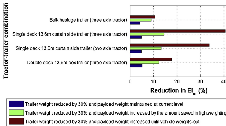
Fig. 9. Estimates of energy consumption reductions that can be achieved through three scenarios involving lightweighting. Note that the third scenario, which involves reducing trailer weight by 30% and increasing the payload until the vehicle reaches its maximum legal GVW (weights-out), will be difficult to achieve for single deck trailers used in grocery distribution because of their volume restrictions. However, this scenario should be achievable in bulk haulage trailers and double-deck trailers used in grocery distribution.
