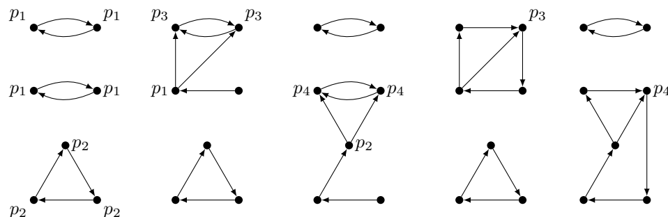
FIG. 9. Impartial probability assignment for five graphs with n = 7 .
