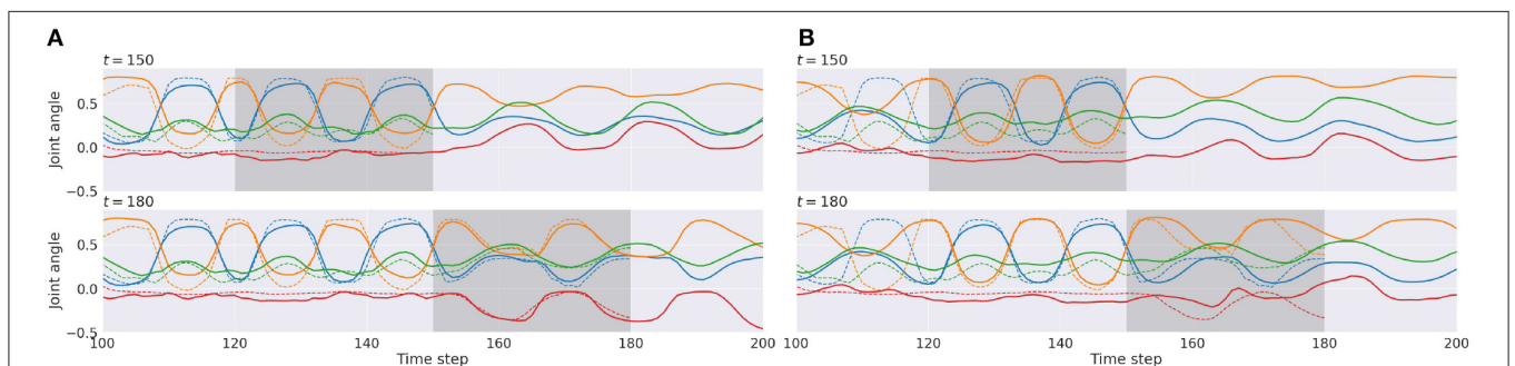
FIGURE 8 | An example of time-series plots of neural activities in the output layer of the proprioception module in the W_1 setting (A) and in the W_5 setting (B). Reconstruction of the past observation and the future prediction at time step 150 (top) and at time step 180 (bottom) are shown. Solid lines represent prediction outputs, and dashed lines represent observations. The shadowed area indicates the error-regression window. For simplicity, only 4 of 16 joint-angles representing movements are shown.
