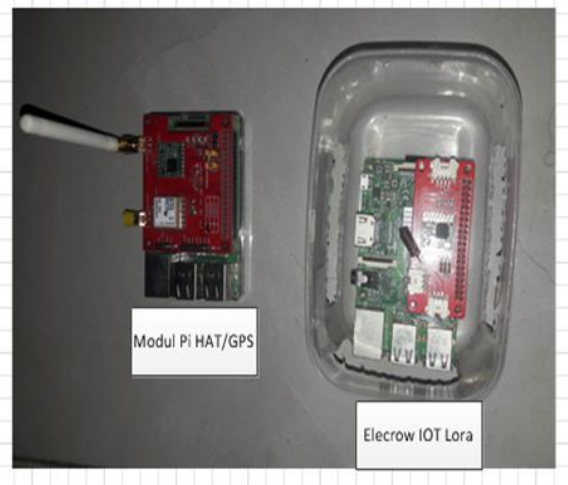
Gambar 4. Lora Gateway
