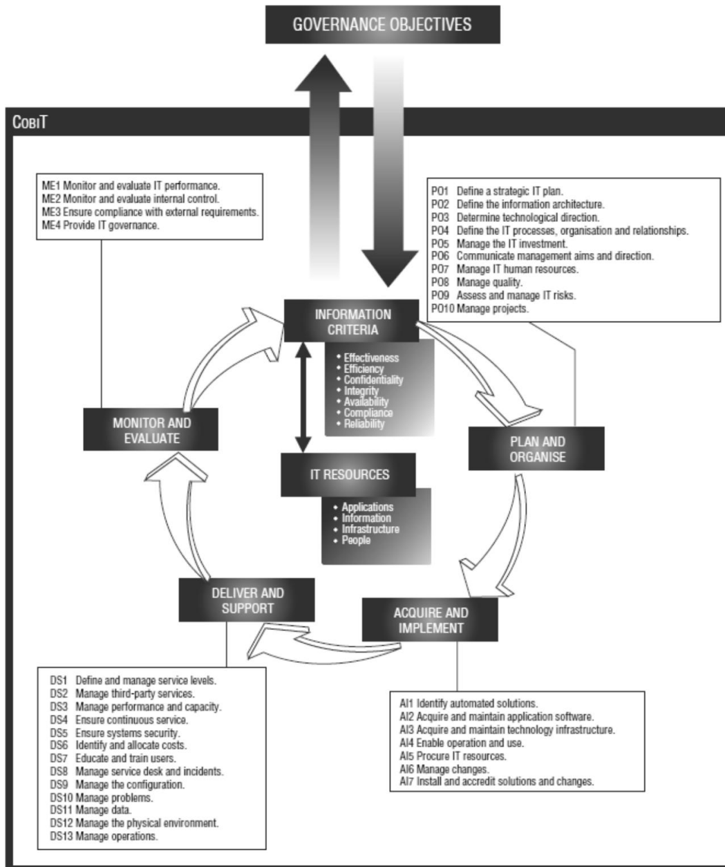
Gambar 1. Framework COBIT 4.1 [2]
