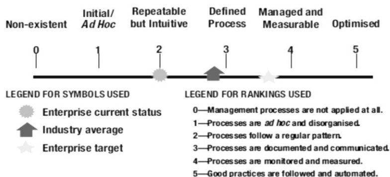
Gambar 2. Maturity model [2]
