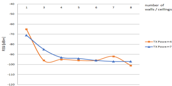
Fig. 19. RSSI versus number of walls / ceilings.
