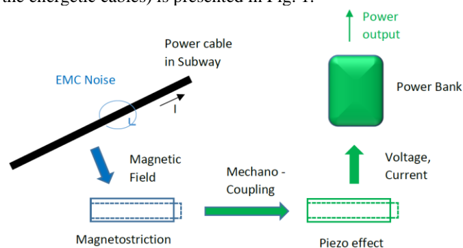
Fig. 1. Example of the Energy Harvesting from the magnetic noise in the Subway [2].
