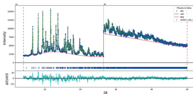
Figure 12 Rietveld plot for (I). The blue crosses represent the observed data points, and the green line is the calculated pattern. The cyan curve is the normalized error plot. The vertical scale has been multiplied by a factor of 5 × for 2\theta > 26.5^\circ . The row of blue tick marks indicates the calculated reflection positions. The red line is the background curve.
