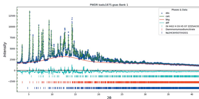
Figure 13 Rietveld plot for (II). The blue crosses represent the observed data points, and the green line is the calculated pattern. The cyan curve is the normalized error plot. The row of blue tick marks indicates the calculated reflection positions. The red and cyan tick marks indicate the reflection positions for the diammonium sodium citrate and diammonium hydrogen citrate impurities. The red line is the background curve.
