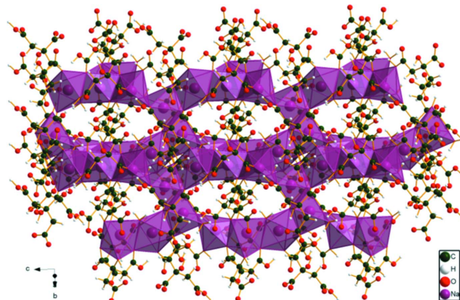
Figure 7 View of the crystal structure of (I), viewed down [\bar{1}10] .
