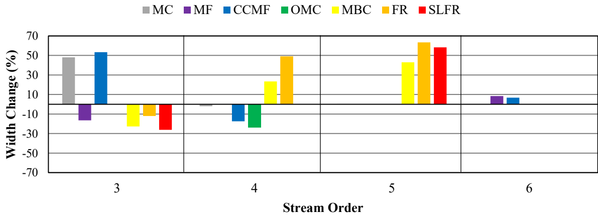
Figure 24. Percent bar width change from 1995 to 2015.
