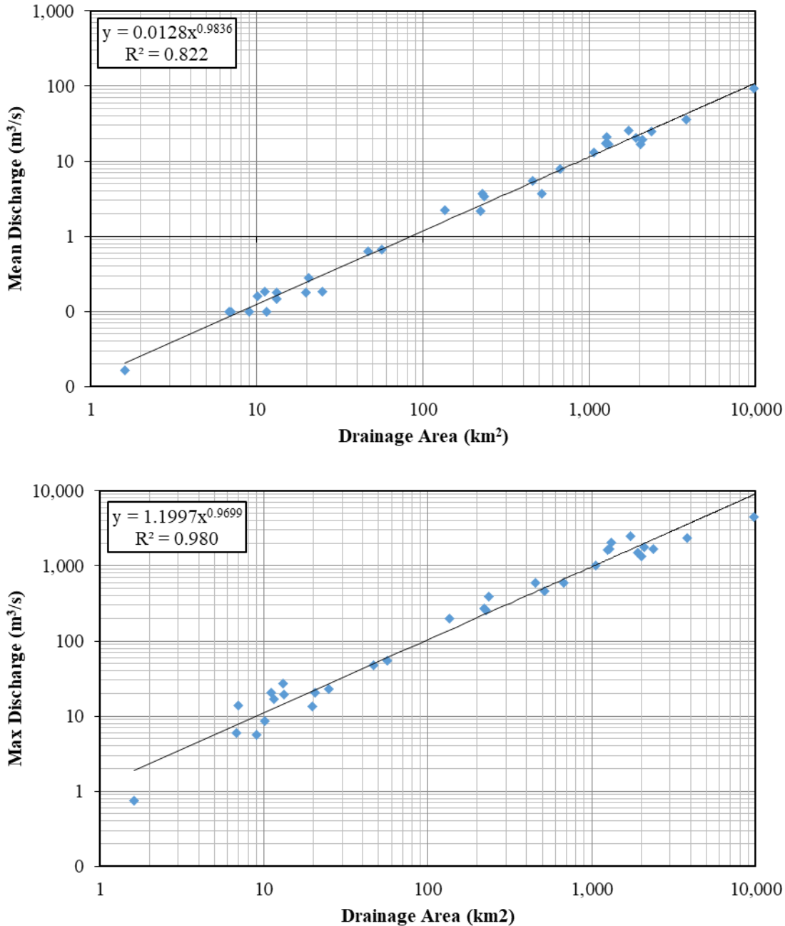
Appendix A-1. Mean and max discharge and drainage area relationships for USGS gaging stations near the study watershed.
