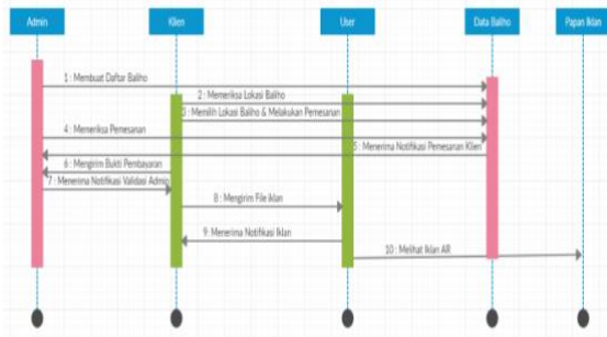
Gambar 3. Sequence Diagram
