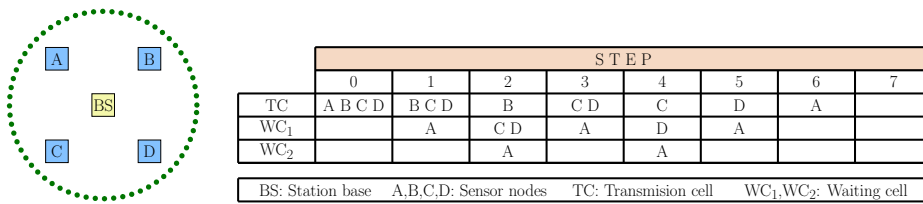
Fig. 3. Collision resolution example using 2CS-WSN with 4 nodes in collision and 2 waiting cells.
