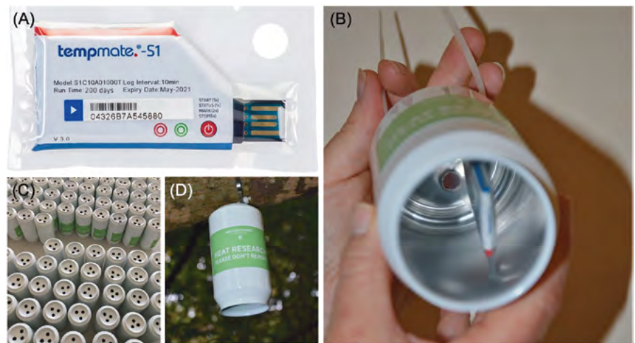
FIGURE 3: Details of the Local Heat Logger designed by Western Sydney University. (A) The sensor used to record near-surface air temperature. (B) The protective shield with sensor inside. (C) Detail of the shield showing the holes necessary for air flow inside the shield. (D) Installation of the Local Heat Logger in the field with the open bottom facing the surface.
