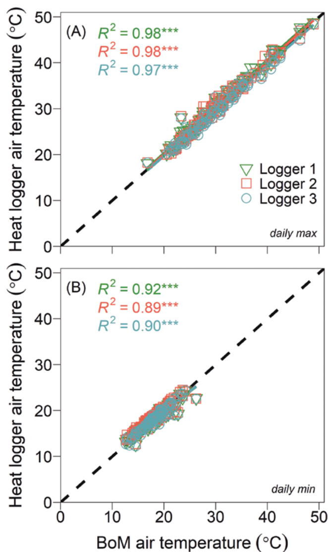
FIGURE 4: Calibrations of near-surface air temperatures measured with three custom-built Local Heat Loggers against data recorded by the Bureau of Meteorology weather station at Penrith Lakes. Daily measurements of (A) maximum and (B) minimum air temperatures for the interval of 14 December 2019 to 30 March 2020 were used in the calibrations. All calibrations yielded highly significant correlations ( p < 0.001 ).
