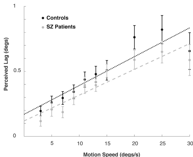
Fig. 2. Average extent to which participants with and without schizophrenia perceived the moving stimulus ahead of the flash at 10 target speeds. Error bars represent standard error.
