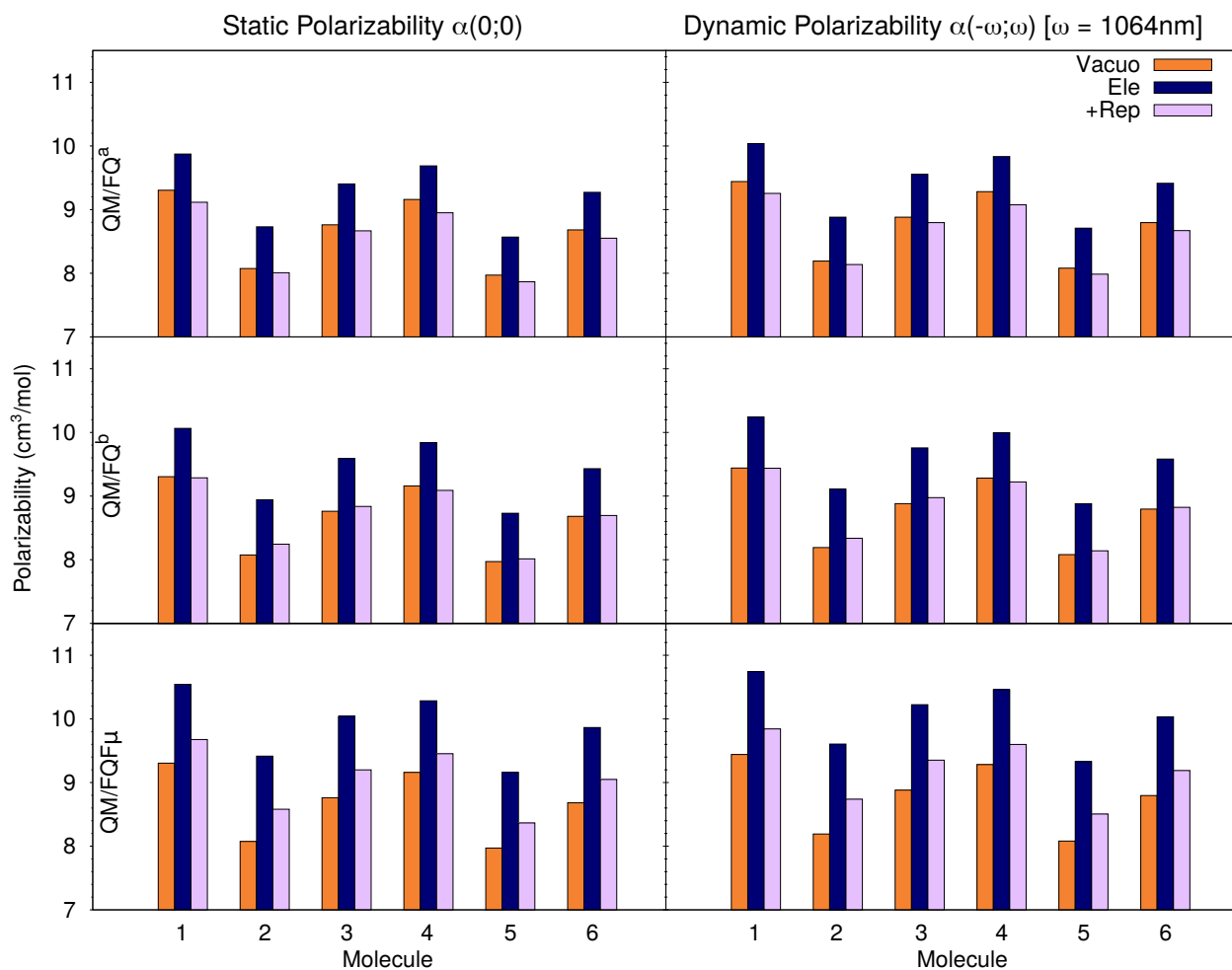
Figure 6: Static (left) and dynamic (right) polarizabilities of molecules 1–6 evaluated at 1064nm in vacuo and in solution (with and without repulsion effects) with three different models for the electrostatic component: FQ^a (top), FQ^b (middle), and FQF_\mu (bottom).
