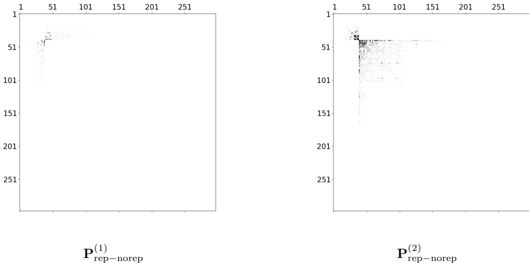
Figure 4: Difference between the density matrix derivatives with and without Pauli repulsion of a randomly snapshot of molecule 1 extracted from MD simulation. The first derivative \mathbf{P}^{(1)} is on the left panel and the second derivative \mathbf{P}^{(2)} is on the right panel. Derivatives are taken with respect to the z component of the electric field.
