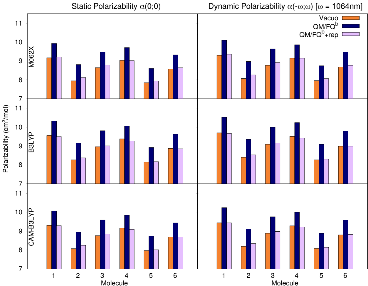
Figure 5: Static (left) and dynamic (right) polarizabilities of molecules 1–6 evaluated at 1064nm in vacuo and in solution (with and without repulsion effects) with three different density functionals: M06-2X (top), B3LYP (middle), and CAM-B3LYP (bottom).
