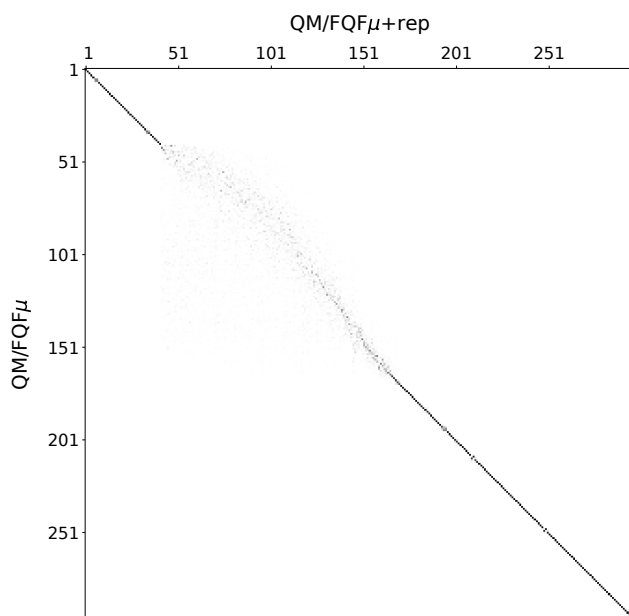
Figure 3: \mathbf{J} matrix of a randomly snapshot extract from MD simulation (see equation 10)
