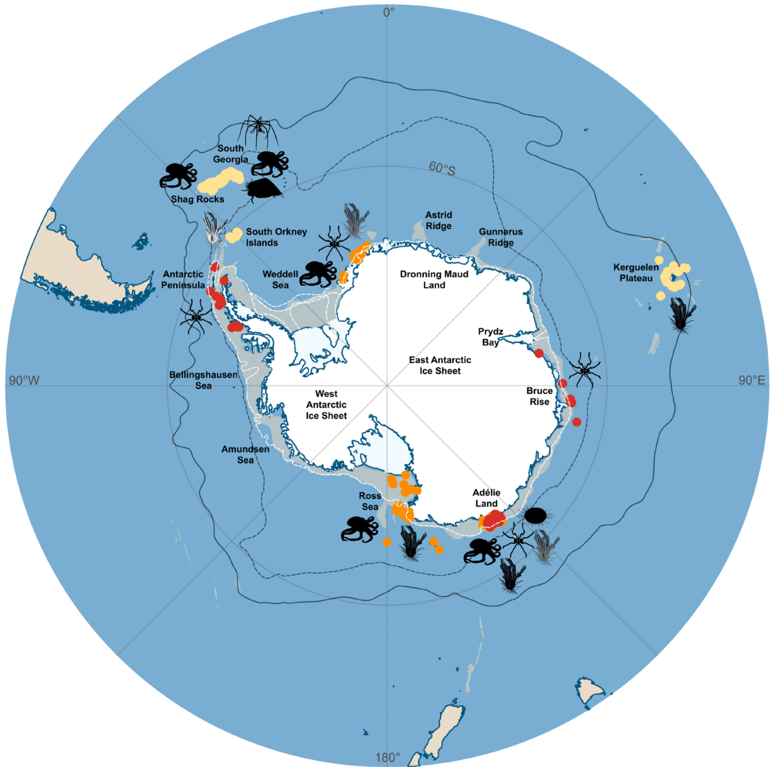
Figure 1. Map of Antarctica and proposed areas of Southern Ocean glacial refugia. Areas of glacial refugia were inferred from the sample locations that were associated with molecular signatures of glacial refugia, with each dot representing a sample location. Each organism on the map reflects the number of times an area was proposed as a refugium for that taxon. Data of grounded ice extent during Last Glacial Maximum (LGM) at 20 ka was extracted from model reconstruction in Bentley et al. (2014). Ice-free areas present on the outer continental shelf during the LGM are observed in the Eastern Weddell Sea, Bellingshausen Sea along Western Antarctic Peninsula, Eastern Ross Sea, between Adélie Land and Bruce Rise in East Antarctica, and Astrid Ridge and Gunnerus Ridge near Dronning Maud Land. SBACC, southern boundary of Antarctic Circumpolar Current; PF, Polar Front.
