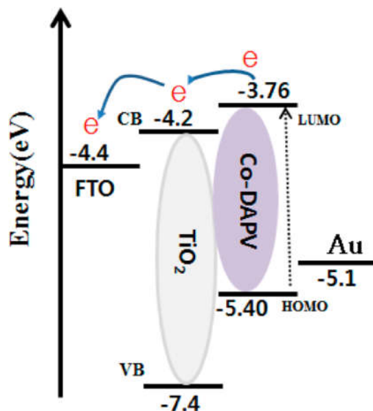
Figure 7. Energy level diagram showing the band edge alignment at TiO 2 -DAPV heterojunction, showing favorable energy cascade for unidirectional charge transfer. Reproduced with permission from [147].
