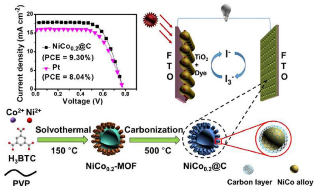
Figure 10. Schematic illustration of the formation process of NiCo 0.2 @C and cell performance. Reproduced with permission from ref. [176].
