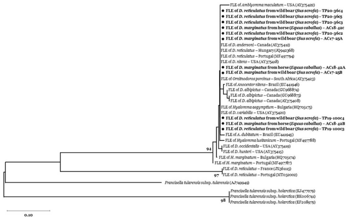
Figure 2. Phylogenetic tree of tul4 (17 kDa lipoprotein) gene of Francisella spp. obtained from 11 nucleotide sequences (200 bp) identified in feeding D. marginatus and D. reticulatus ticks, respectively collected from horse and wild boar in our study areas (AC: Alpi Cozie regional park; TP: Po Torinese natural park). Reference sequences are identified by GenBank accession number enclosed in parentheses. Bootstrap values (1000 replications) above 70 are shown next to the internal nodes. Amplicons from this study are indicated with a black circle (●).
