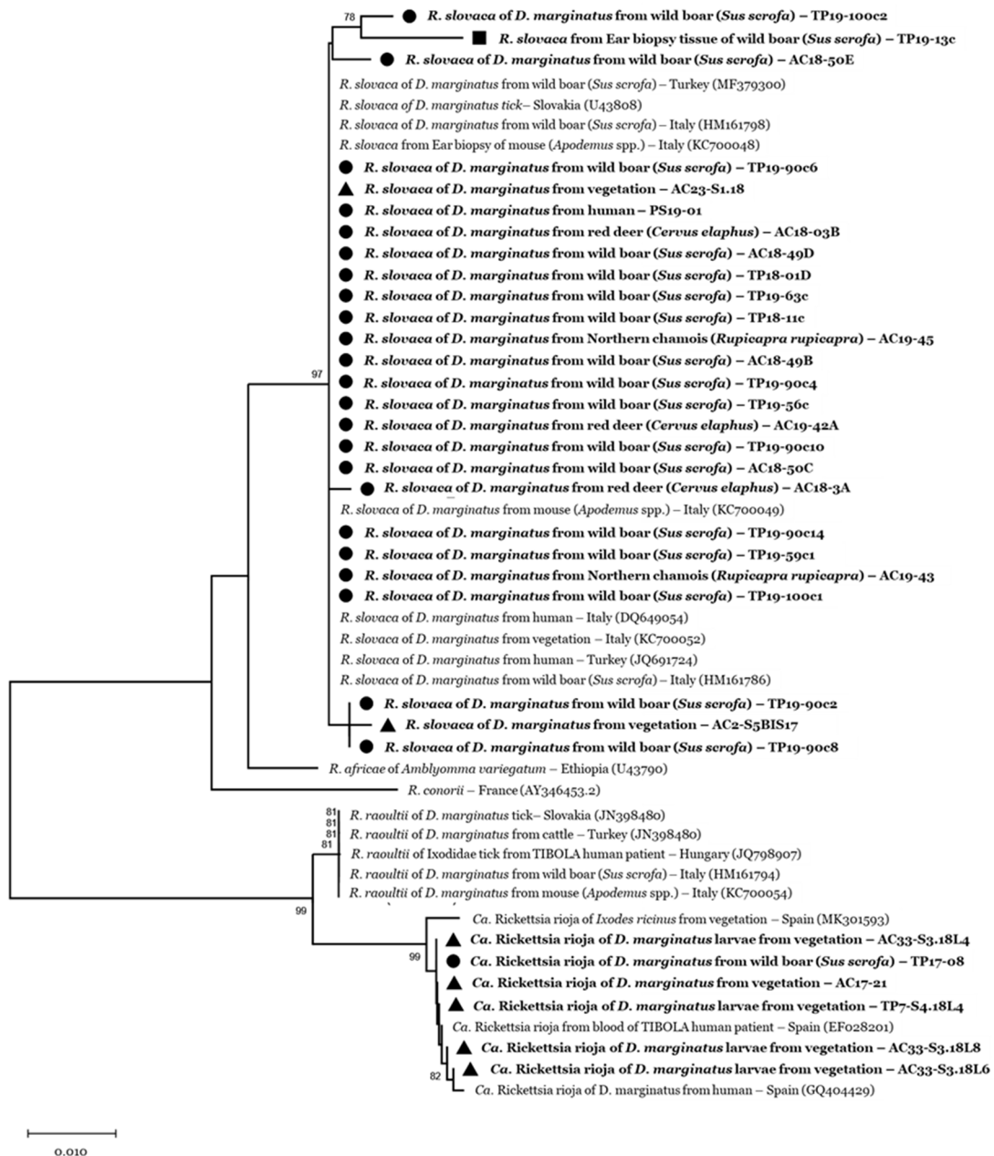
Figure 1. Phylogenetic tree of OmpA gene of Rickettsia spp. obtained from 32 nucleotide sequences (426 bp) from D. marginatus and D. reticulatus ticks collected in the study areas (AC: Alpi Cozice regional park; TP: Po Torinese natural park). Reference sequences are identified by the GenBank accession number enclosed in parentheses. Bootstrap values (1000 replications) above 70 are shown next to the internal nodes. Amplicons obtained in this study are indicated with a black symbol: ● Feeding ticks from wild boar, red deer, Northern chamois, and humans; ▲ Dermacentor ticks collected from the vegetation; and ■ Ear biopsy collected from wild boar.
