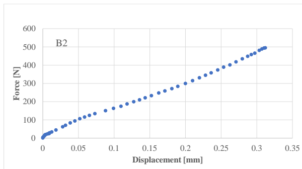
Figure 5 The graph shows the pull-out test on nail B2. In this case the nail was free to move through the crossbeam (the graph shows no initial steep increase of the force, which would be caused by friction or adhesion between nail shank and crossbeam), and a linear correlation is observed between the force and the displacement.
