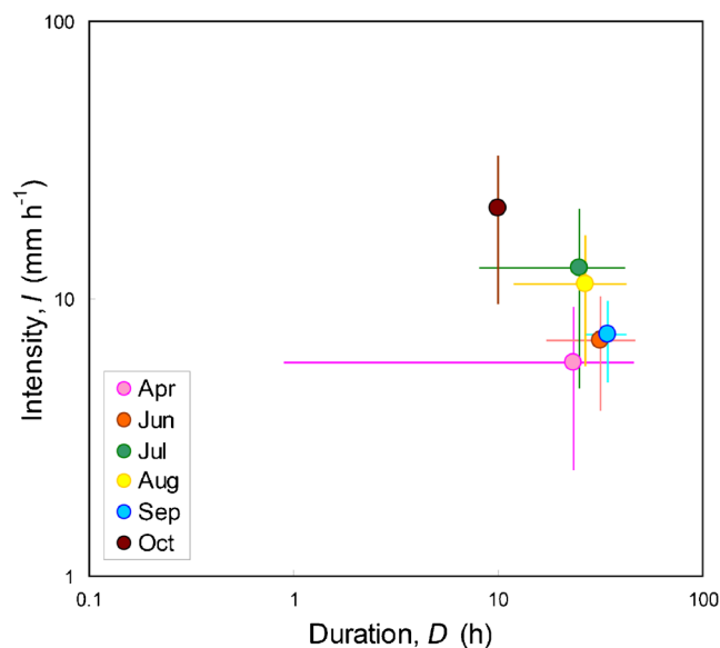
Fig. 11 Differences in the average I - D conditions demonstrated by the monthly classification of landslide occurrence during 1963–2018. The mean (with minimum–maximum) of absolute antecedent rainfall of the months preceding each landslide occurrence month is 133 mm (48–279 mm) from January to March for landslides in April; 337 mm (173–518 mm) from January to May for landslides in June; 492 mm (236–892 mm) from January to June for landslides in July; 770 mm (471–1201 mm) from January to July for landslides in August; 1026 mm (700–1497 mm) from January to August for landslides in September; and 1178 mm (742–1755 mm) from January to September for landslides in October during 1963–2018. Error bars indicate standard deviations
