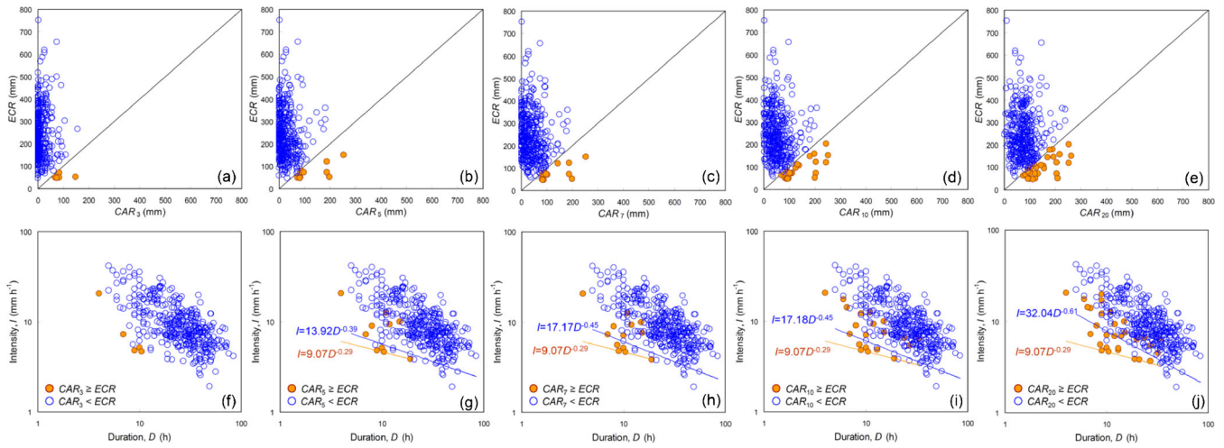
Fig. 8 Relationships between event cumulative rainfall (ECR) and calibrated antecedent rainfall (CAR), and differences in I - D thresholds by the relationship between event cumulative rainfall (ECR) and calibrated antecedent rainfall (CAR) for 3 (a, f), 5 (b, g), 7 (c, h), 10 (d, i), and 20 (e, j) days
