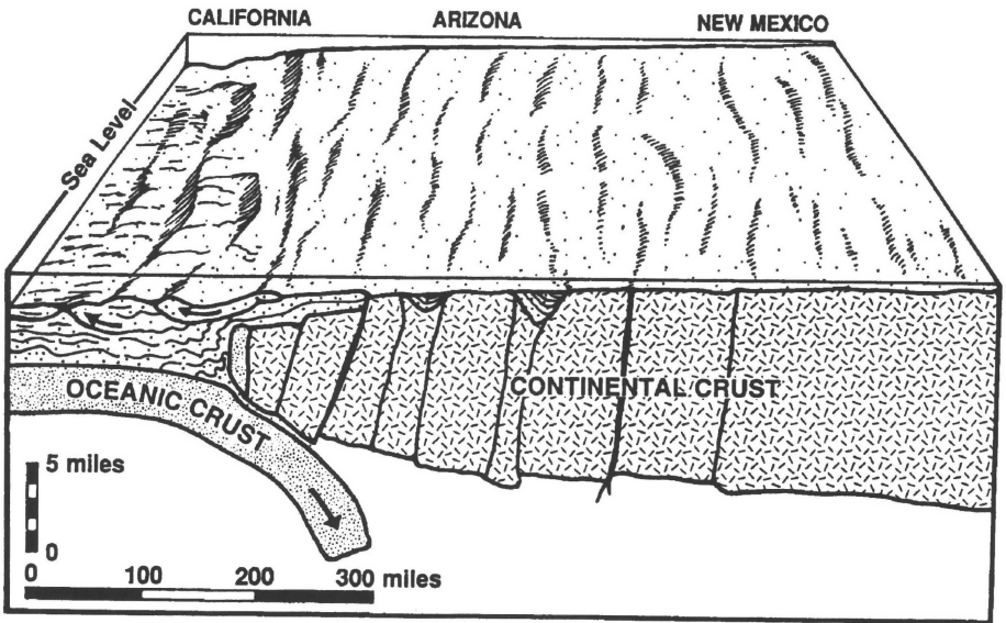
Figure 2. A tectonic-sedimentary model for the beginning of the Flood in the southwestern United States.
